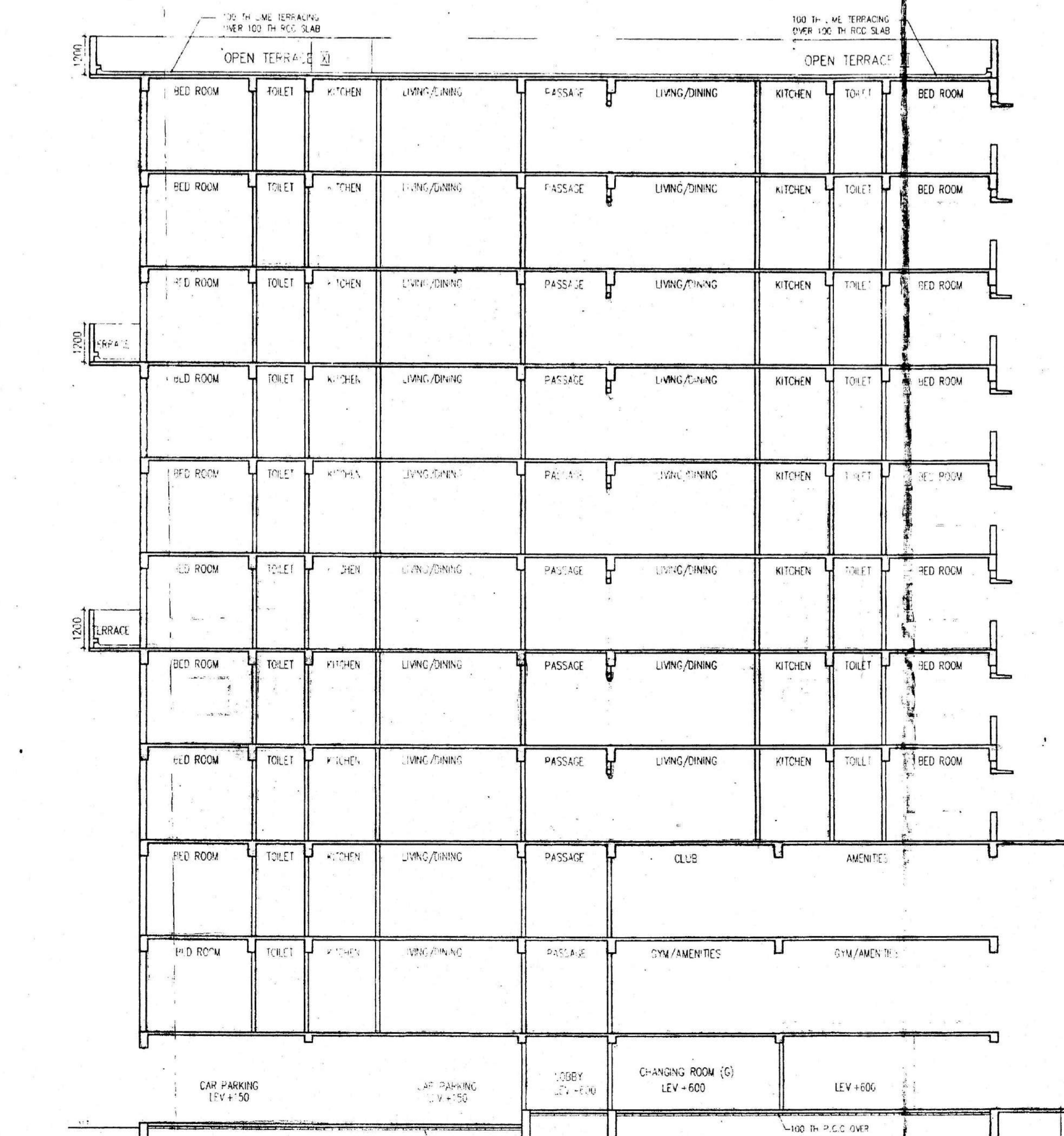
SECTION N-N
