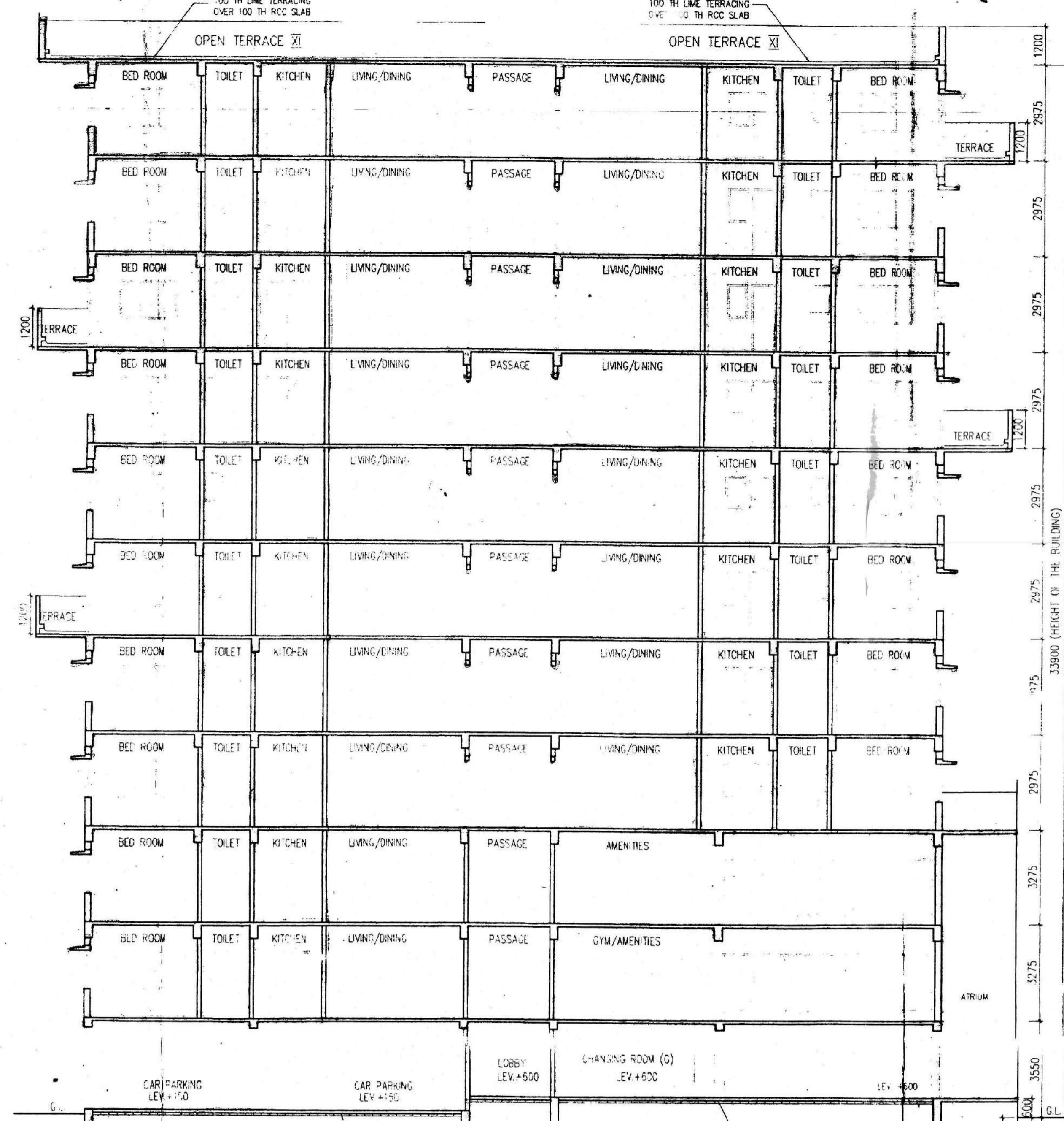
SECTION M-M
