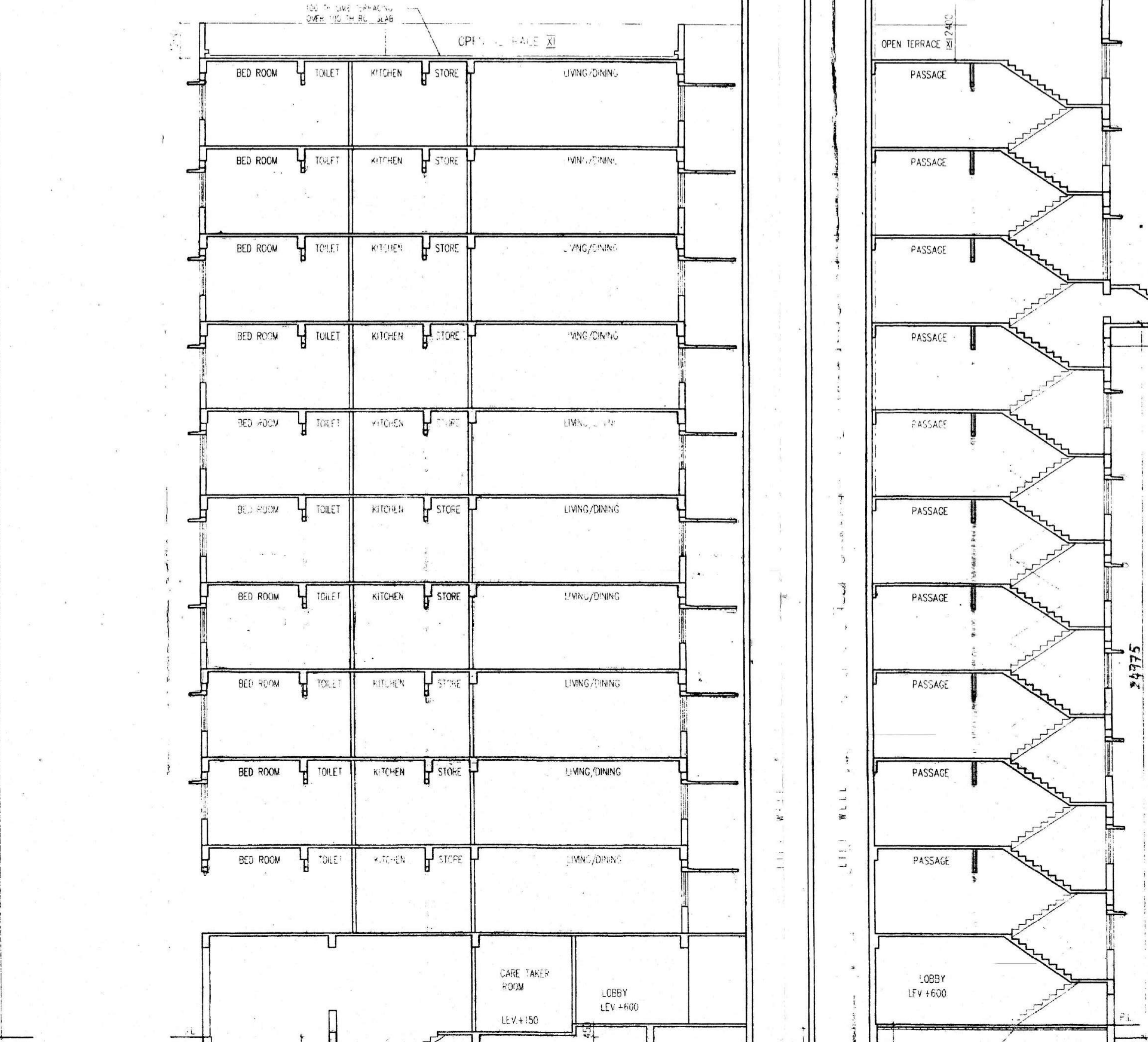
SECTION I-I
