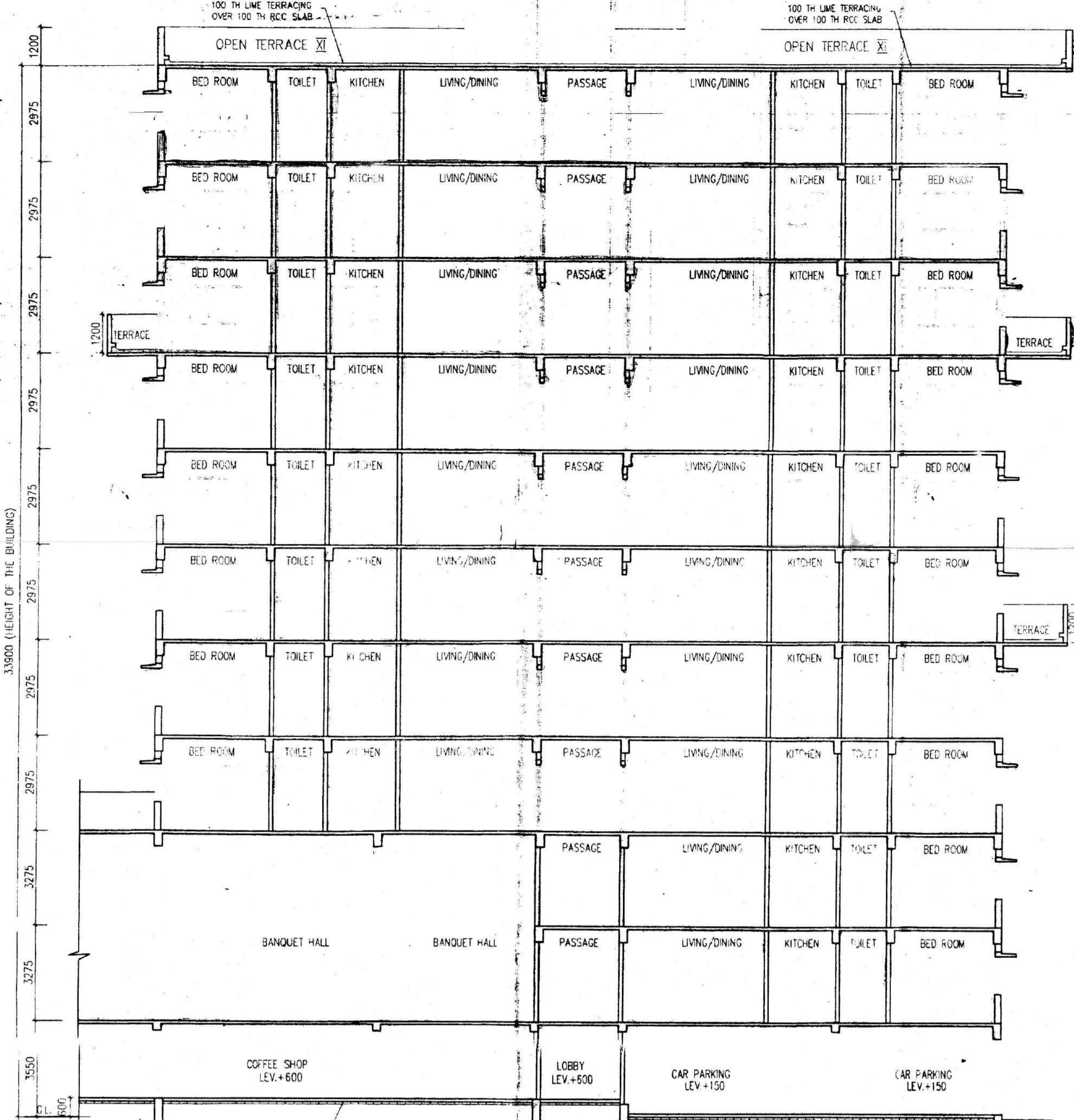
SECTION K-K
